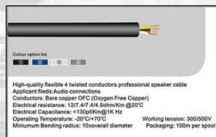
BULK CABLE / 4 & 8 CONDUCTOR
