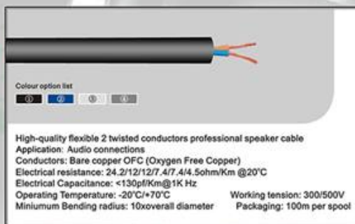
Cable specifications
