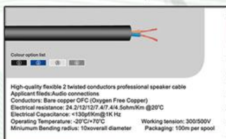
BULK CABLE / 2 CONDUCTOR
